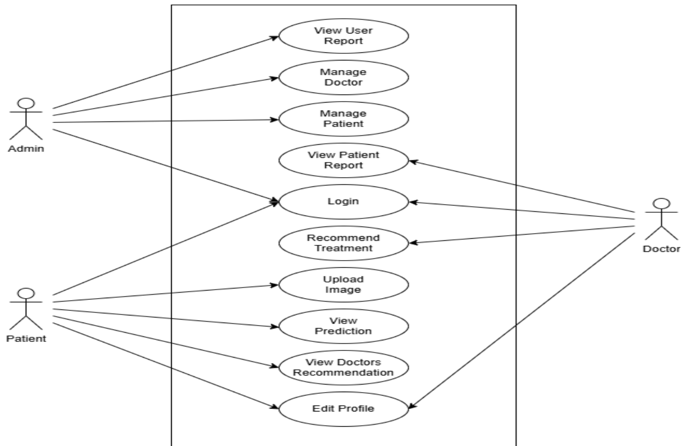
Fig 5.1 Use Case Diagram of Lung Cancer Prediction System Using CNN
