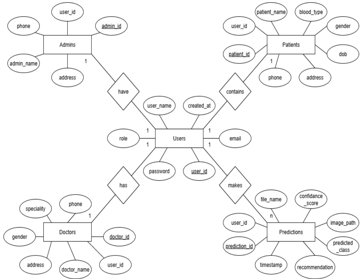
Fig 5.7 E-R Diagram
