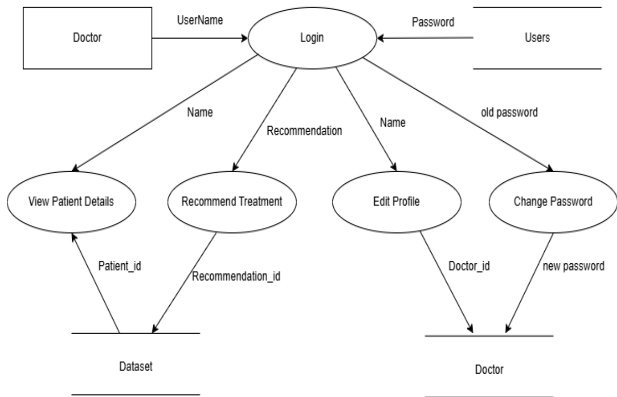
Fig 4.3 Doctor DFD
